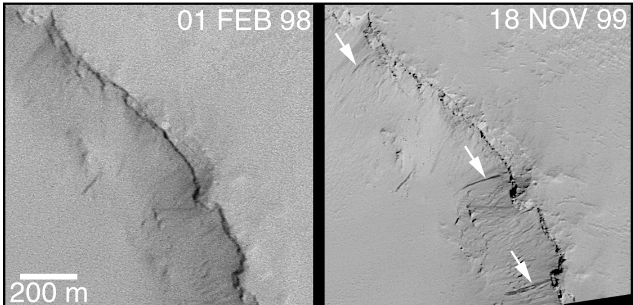
Figure 2. Appearance of 3 new dark slope streaks (arrows) after a 0.92 Mars year interval. Image on left is subframe of MGS MOC AB1-11304, image on right is M09-04872. These are located in a crater at 6.0°S, 183.8°W. Both views are illuminated from the lower right, north is toward the left.
