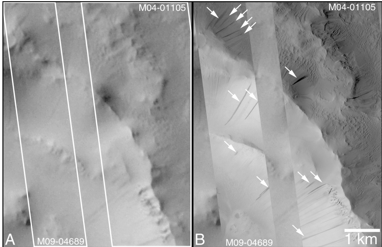
Figure 1. Appearance of new dark slope streaks over 11 Mars year interval. (A) On the left is a subframe of Viking orbiter image 748A12 taken in May 1978. White outlines indicate the location of two MOC images obtained in 1999. (B) On the right are the two MOC image subframes (M09-04689 from November 1999, and M04-01105 from August 1999) overlain on the earlier Viking image. New dark slope streaks are indicated by arrows. Location is a crater at 1.8°S, 343.9°W. North is up, illumination is from the left.
