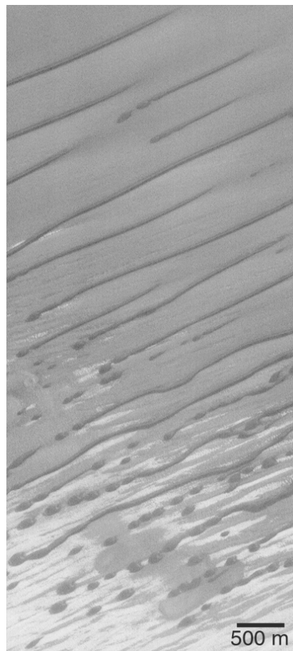
Figure 4. Linear dunes associated with extended barchans in Chasma Boreale near 84.2^{\circ}\text{N} , 37.6^{\circ}\text{W} . Illumination is from the upper left. Bright areas are frost. MOC image M03-07330, taken near the evening terminator in early northern autumn on 7 August 1999.
