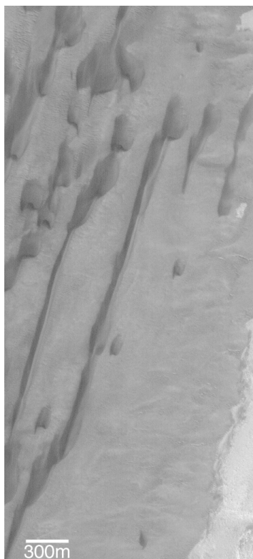
Figure 1. Seif dunes formed from elongated barchans in a trough in southern Chasma Boreale. Illumination is from the lower right. Sub-frame of MOC image M01-00179, near 82.2^{\circ}\text{N} , 76.7^{\circ}\text{W} , taken 6 May 1999.
