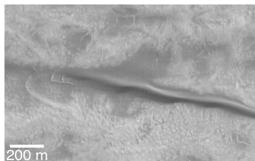
Figure 3. Single, semi-sinuous longitudinal dune near 83.0^{\circ}\text{N} , 204.0^{\circ}\text{W} , close to the margin of the permanent north polar cap. The somewhat sinuous form of this dune resembles the dunes in classic seif dune studies in the Negev Desert by H. Tsoar (see Fig. 1 of [8]). Sub-frame of MOC image M02-01955, illuminated from the upper right, acquired on 15 June 1999.
