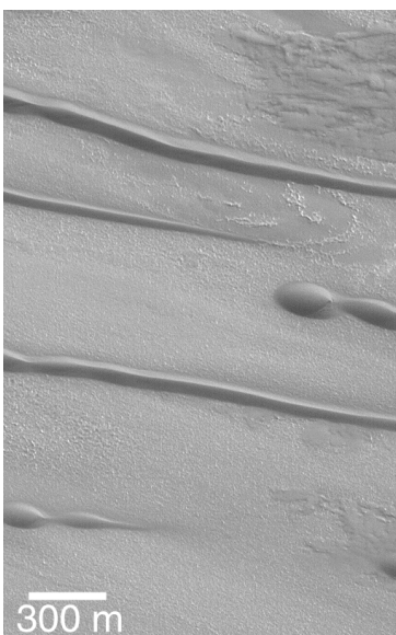
Figure 2. Seif dunes formed and forming from barchan dunes in Chasma Boreale near 84.8^{\circ}\text{N} , 26.2^{\circ}\text{W} . Sub-frame of MOC image M02-00783, illumination from the upper right. Image obtained 8 June 1999.
